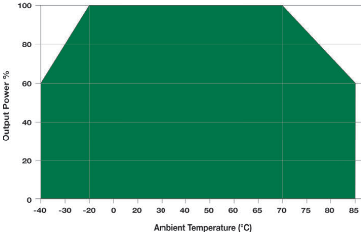
Derating Curve, 85 -110 VAC, 70 - 130 VDC
