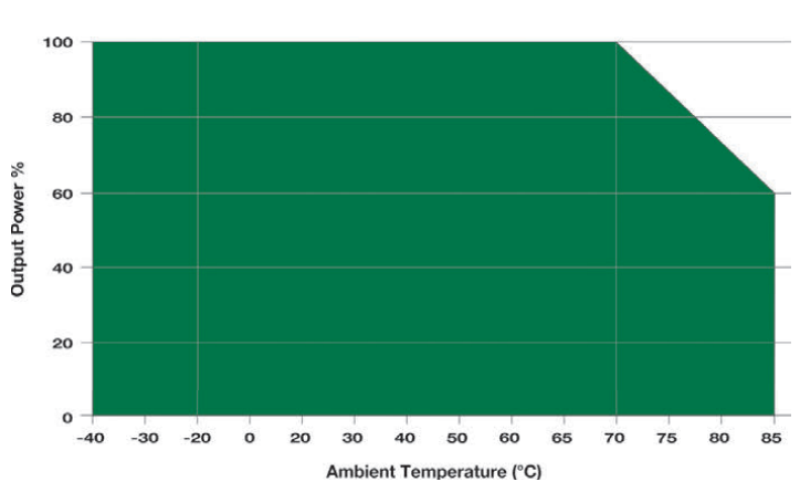
Derating Curve, 110 -305 VAC, 130 - 430 VDC
