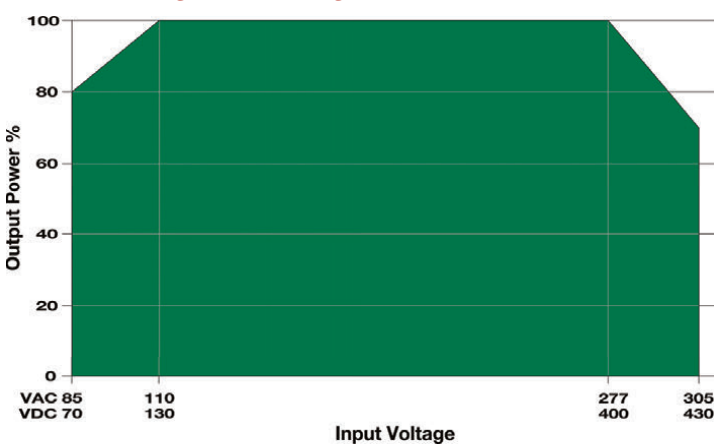
Input Voltage Derating, At +25°
