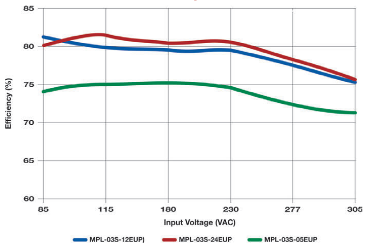
Efficiency vs Input Voltage VDC Input
