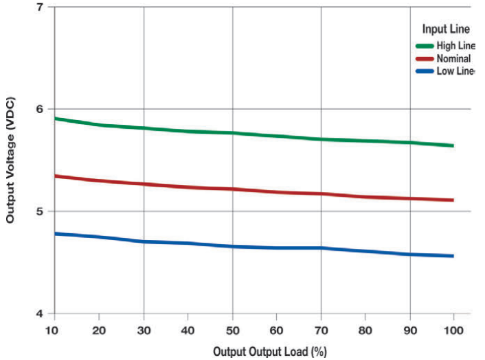
Output Voltage vs Load: MH0548S-05
