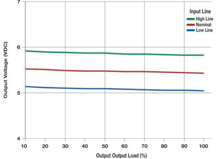
Output Voltage vs Load: MH0548S-05
