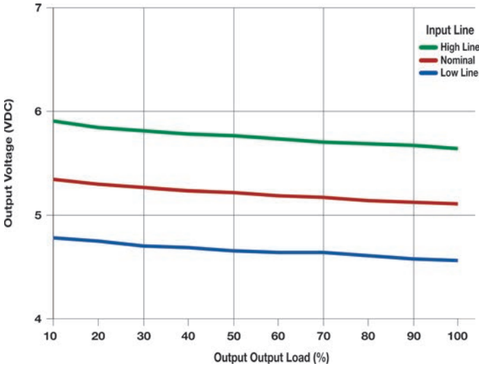
Output Voltage vs Load: MH0524S-05
